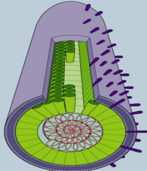
Rabies virus
