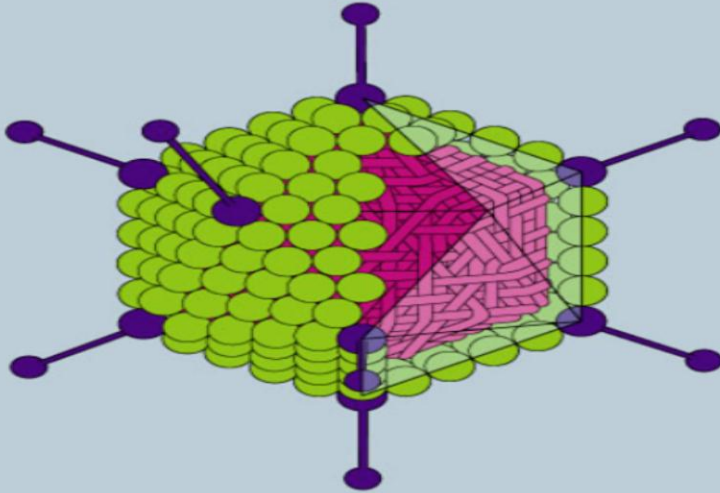
Adenovirus
